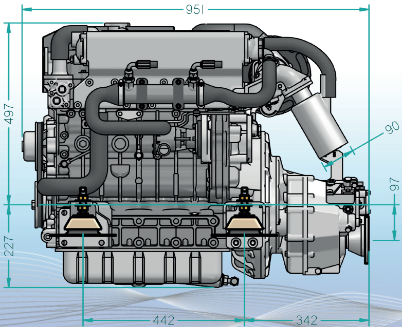
These are typical dimensions: visit our website for all engine / gearbox option drawings or contact Beta Marine direct
