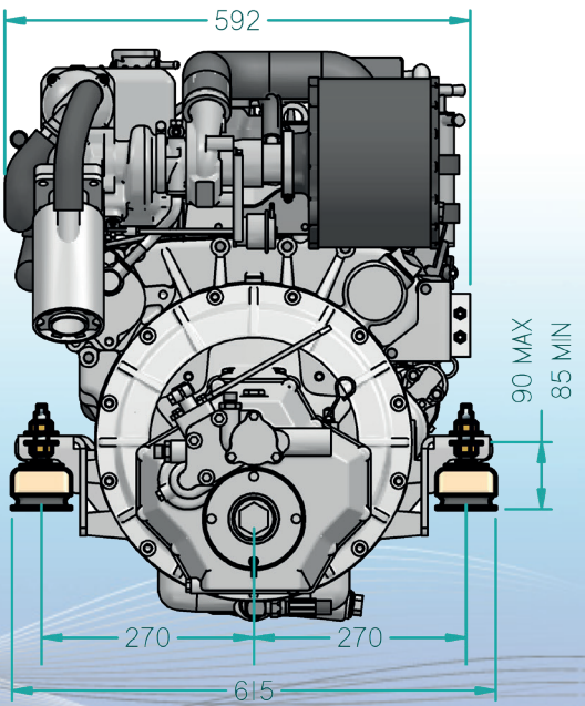
These are typical dimensions: visit our website for all engine / gearbox option drawings or contact Beta Marine direct
