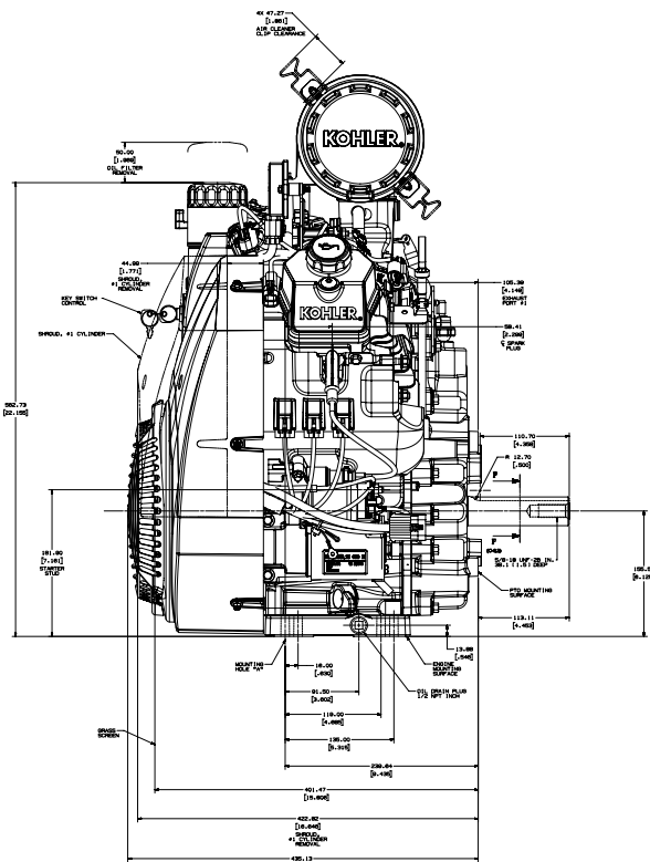
Starter side view
