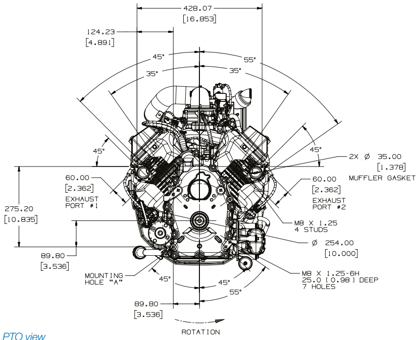
PTO view
