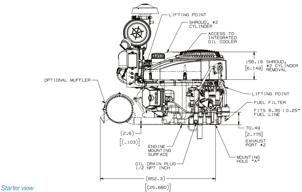
Starter view
