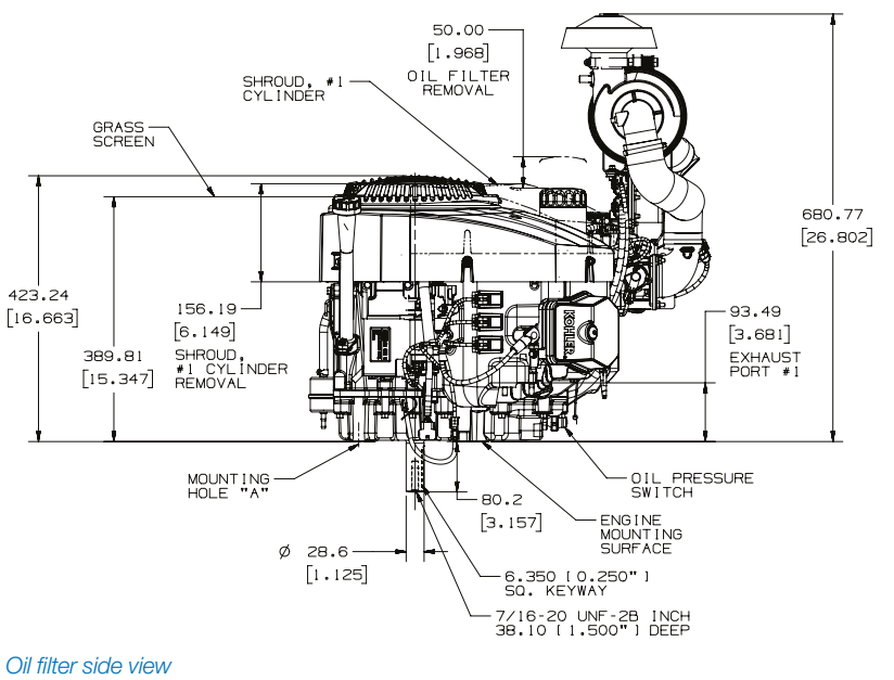
Oil filter side view
