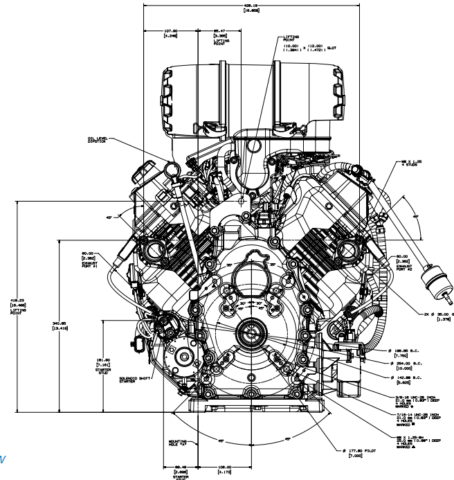
PTO view
