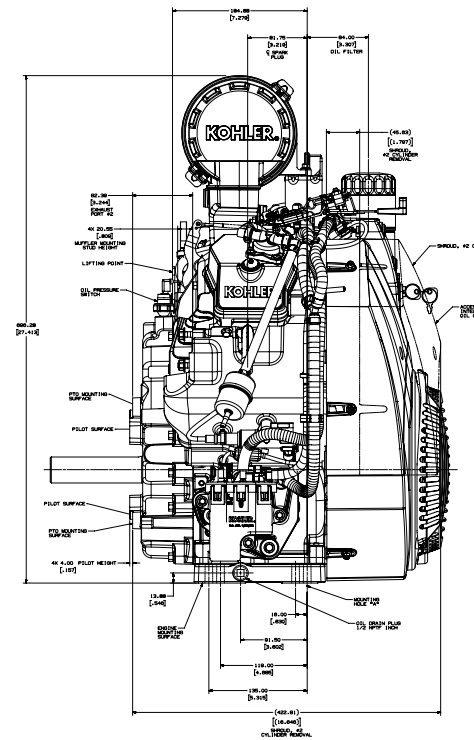
Oil filter side view
